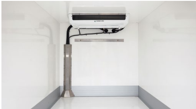
Thermo King V-520 Max or Carrier 40 XR Refrigeration Unit
