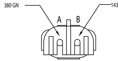
16.2 CONNECTOR, 2-WAY WEATHER PACK SHROUD 12010973
