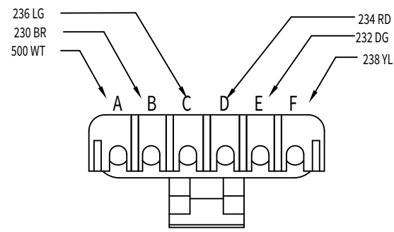
1.1 TO REAR STRUCTURE HARNESS 12015799
