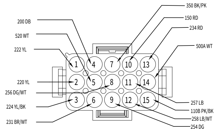
2.1 TO ROOF HARNESS 770023-1
