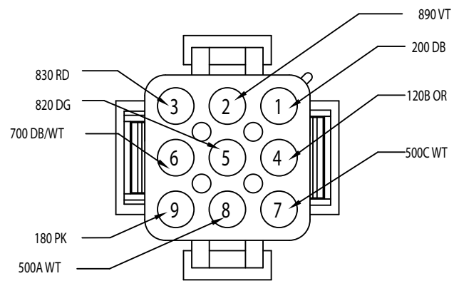
10.4 POWER FEED #2 770021-1
