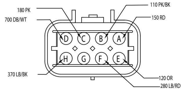
10.1 BODY BUILDER CONNECTOR 15326655
