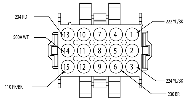
11.1 TO "A" PILLAR HARNESS 770030-1
