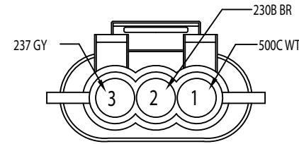
7.8/L LEFT TURN/MARKER LIGHT 282087-1
