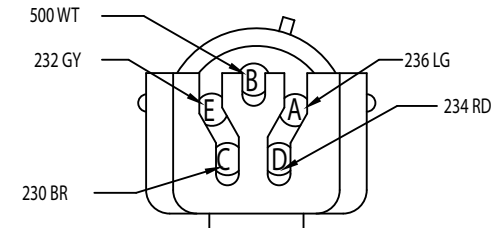
8.1/R RIGHT S/T/T DIST. 12065158
