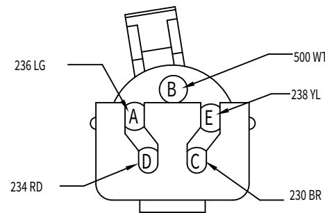
5.1 LEFT S/T/T FEED 12034342
