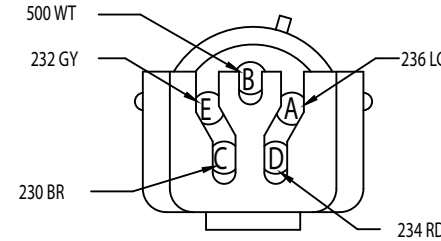
8.1/L LEFT S/T/T DIST. 12065158
