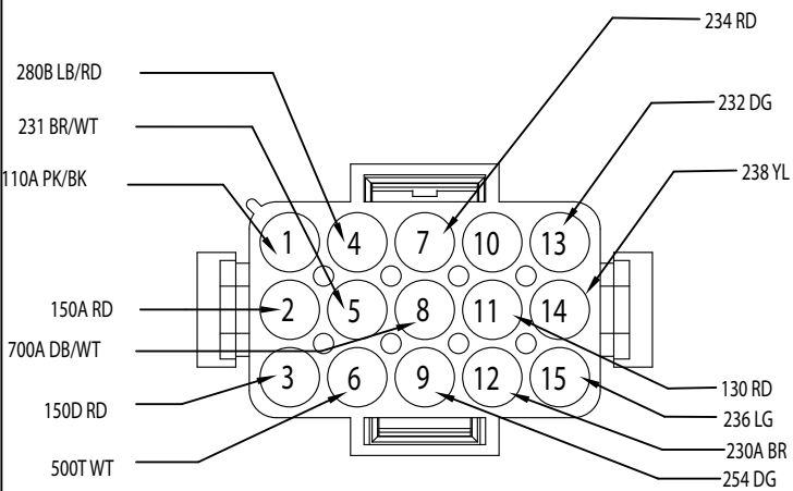
10.3 POWER FEED #1 770023-1
