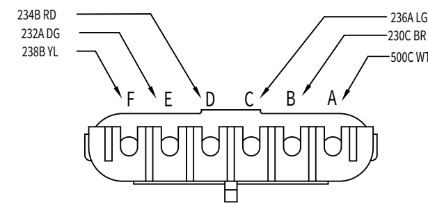
5.4 FRAME RAIL HARNESS 12010975
