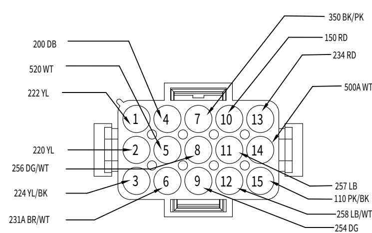
2.2 TO ROOF HARNESS 770023-1
