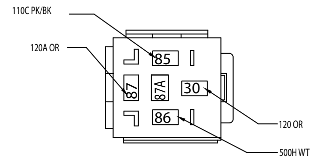
10.6 WIPER POWER RELAY 12033871
