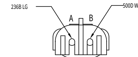
5.5 BACK UP ALARM 12010973
