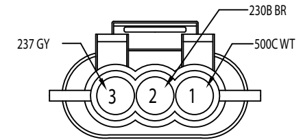
7.8/R RIGHT TURN/MARKER LIGHT 282087-1
