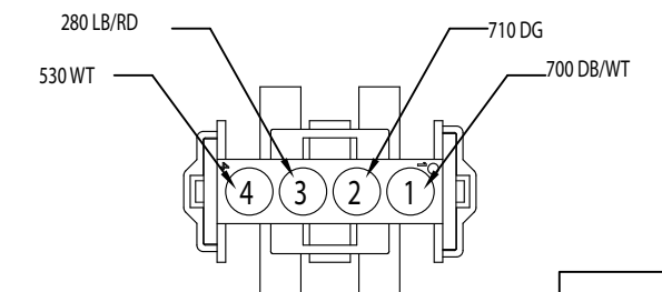
13.1 TO MAIN DASH HARNESS 770026-1
