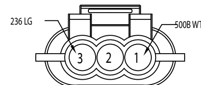
8.3/L LEFT BACK-UP 282087-1
