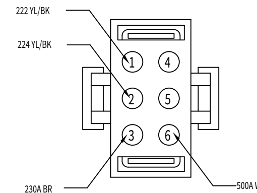
4.4 ROOF HARNESS 770020-1
