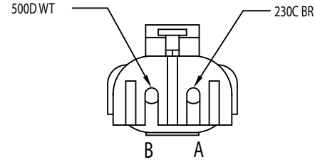
7.9/R RIGHT SIDE MARKER LIGHT 12015792
