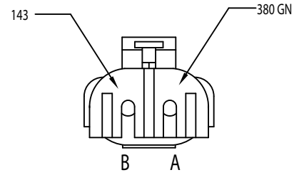
16.1 CONNECTOR, 2-WAY WEATHER PACK TOWER 12015792
