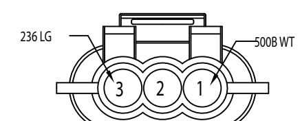
8.3/R RIGHT BACK-UP 282087-1
